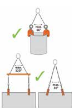
Horizontal plate clamp
